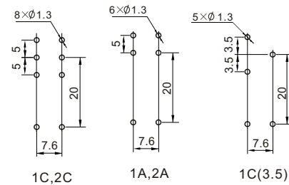
Mounting (Bottom view)
