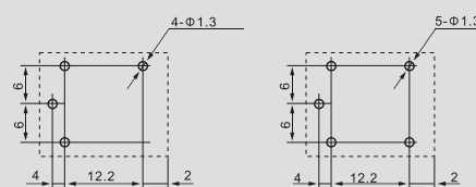
JZC-22F Mounting holes (Bottom view)
